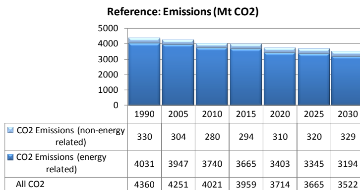
FIGURE 34: CO 2 EMISSIONS
